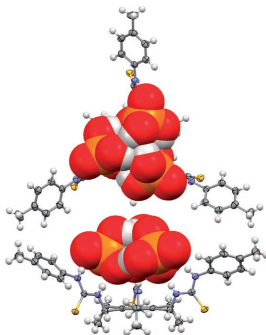
Figure 2. Top and side view of S5-3TBA-3H 2 PO 4 , determined by X-ray crystallography. S5 is shown as thermal ellipsoids at the 50% probability level, while dihydrogen phosphate anions are in a space-filling form. The TBA cations have been omitted. The complex shows C_3 symmetry.
